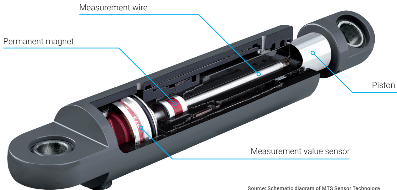
Source: Schematic diagram of MTS Sensor Technology
