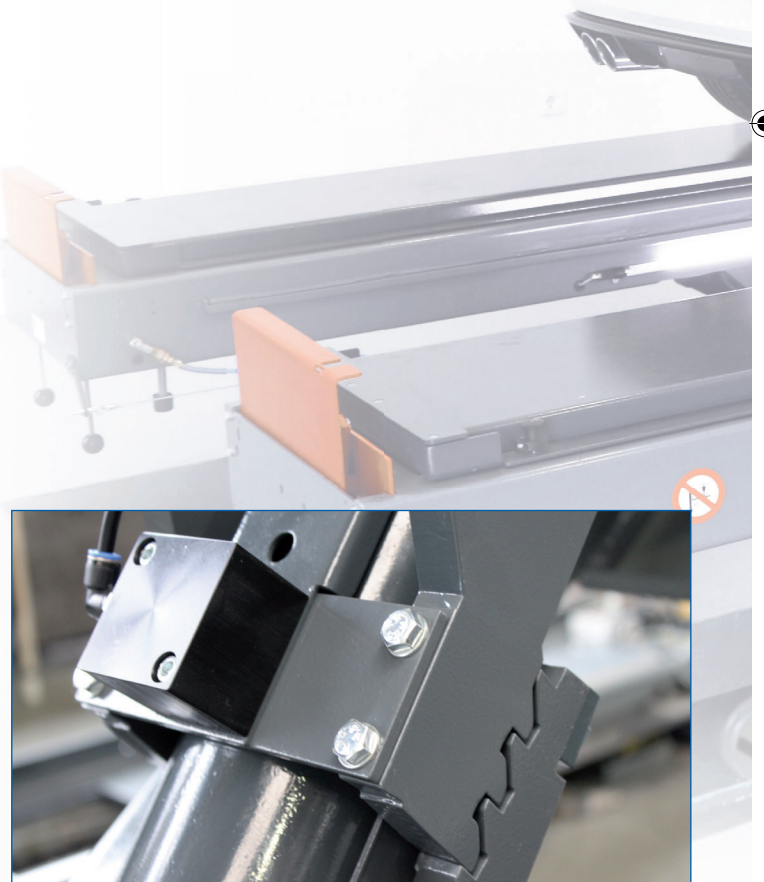
The tothing of the mechanical locks for wheel alignment lifts is machined by milling (option "Lowering Device"). This ensures high measuring accuracy at different working heights.
