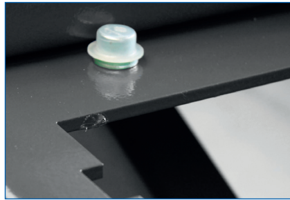
Numerous metal contact surfaces are separated from one another by synthetic/rubber elements.
