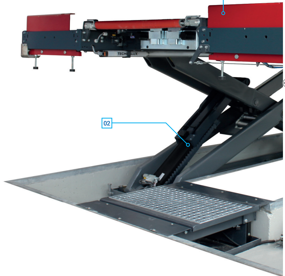
High-powered drive unit – designed for extremely large number of lifting cycles.
